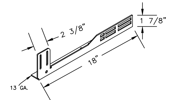
20366 & 7 FLAG BRACKET
